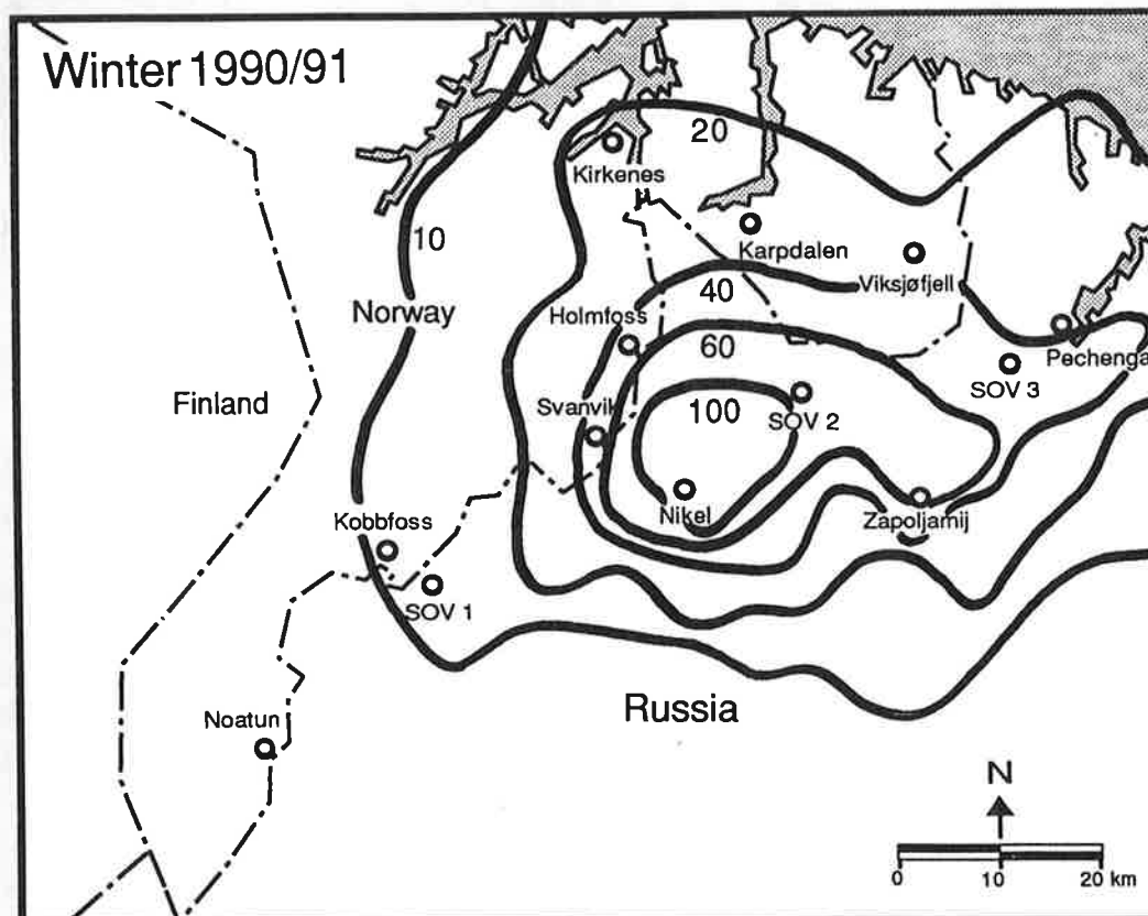
Figure 4: Estimated 6 month average SO_2 concentrations ( \mu g/m^3 )
