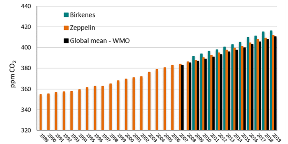
Figure 1: Annual mean value for carbon dioxide (CO 2 ) on Zeppelin (orange bars) and Birkenes (green bars), compared to global mean value from the World Meteorological Organization, WMO (black bars). Source: NILU / Norwegian Environment Agency
