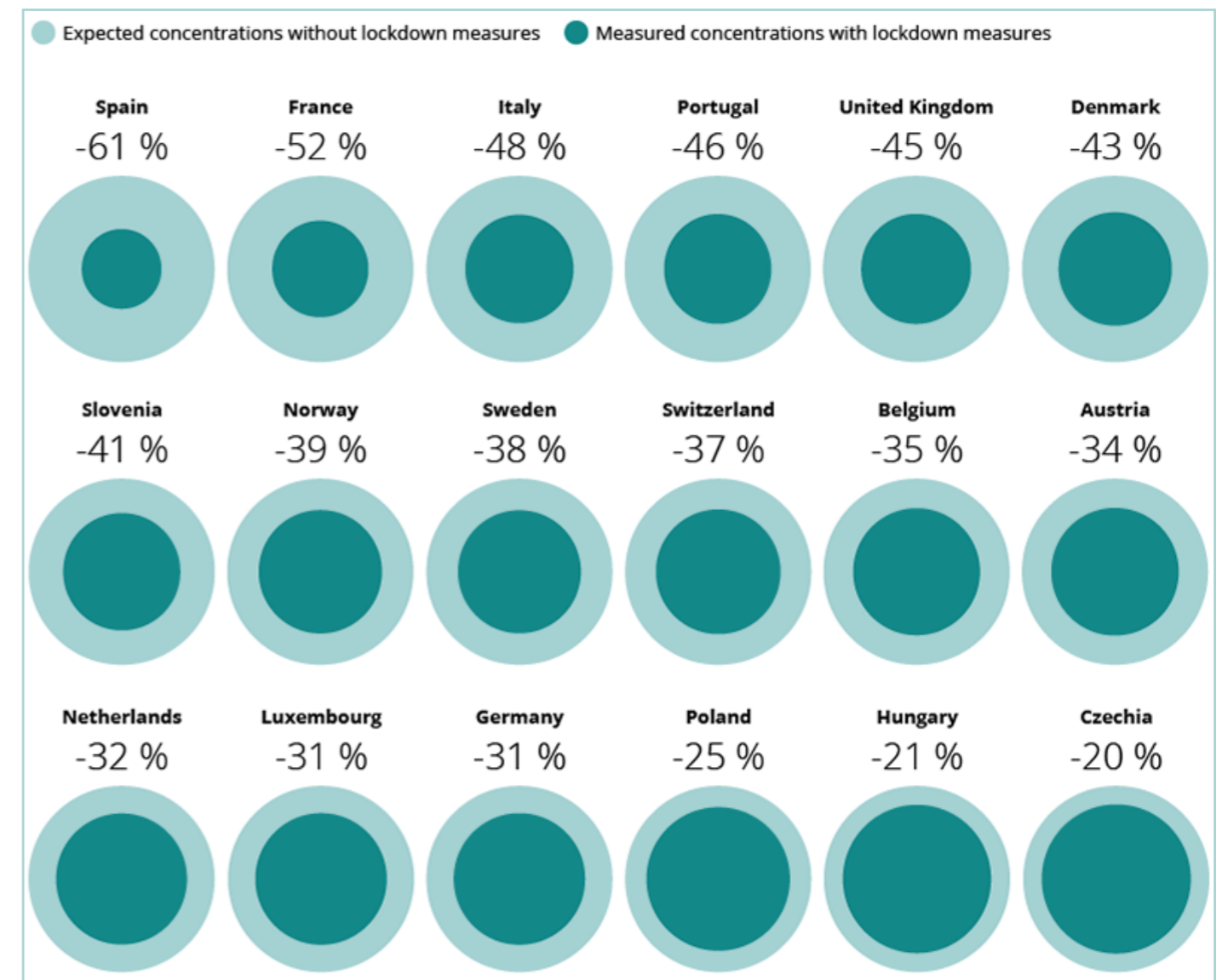
Fig. 5: The figure shows the calculated changes in NO 2 concentrations in a selection of European countries in April 2020. Source: EEA briefing “COVID-19 and Europe’s environment: impacts of a global pandemic”.
