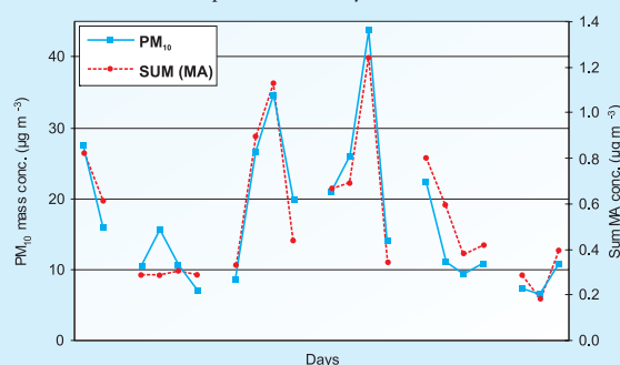
Figure 2: PM_{10} mass concentration and \Sigma MA concentration at Elverum during weekdays. Average temperature in the sampling period was -5.1^\circ C ( -25.7 - 5.6 ). The high degree of correlation indicates that wood burning is the dominating source.
