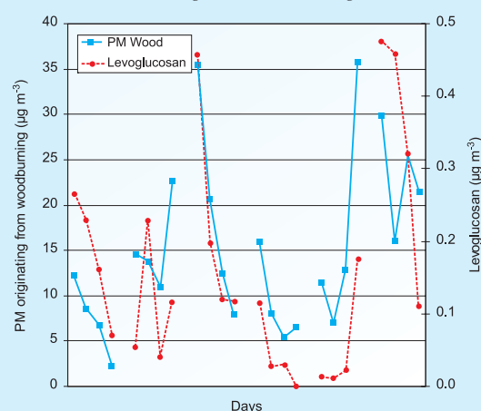
Figure 3: Comparison between levoglucosan and modeled concentrations of particulate matter due to wood burning contributing to the PM_{10} fraction on weekdays in Oslo. The discrepancies between the two datasets indicates that there are certain conditions that the model is not accounting for. R^2 is 0.39 and r_p = 0.63
