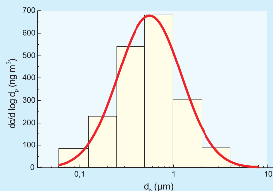
Figure 1: Particle size distribution of \Sigma MA measured in ambient air at Elverum, using a Berner cascade impactor. The line is the lognormal fit to the observed data given by bars. The mode diameter ( x_c ) of the log normal distribution is 561 nm. 80% of the \Sigma MA is associated with particles < 1 \mu m .
